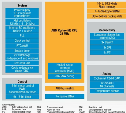
STM32 Value line block diagram
