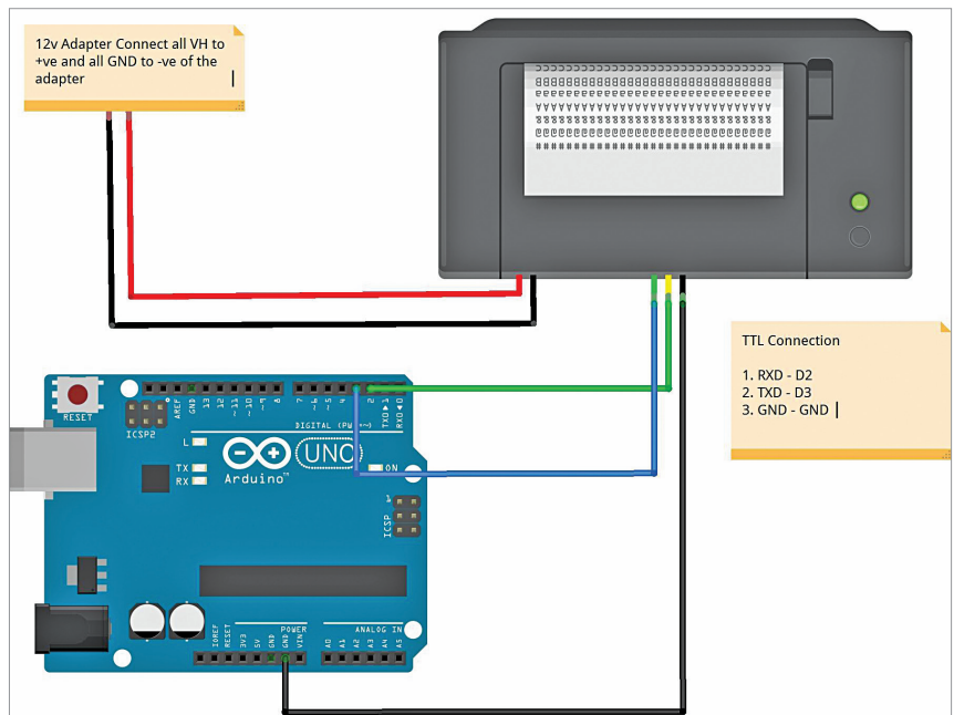
Fig. 2: Circuit diagram
