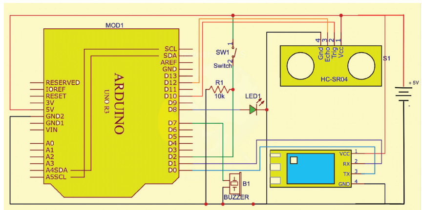
Fig. 1: Circuit diagram
