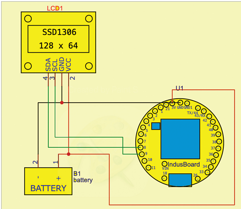
Fig. 6: Circuit diagram
