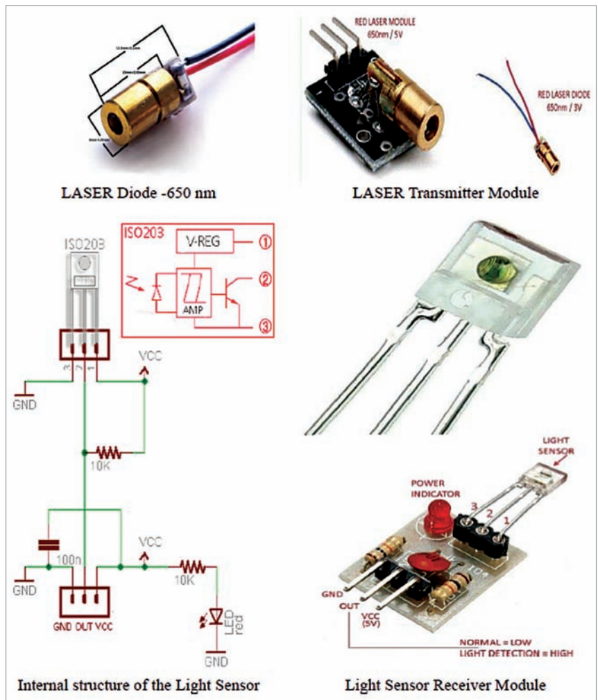
Fig. 4: Laser light sensor assembly
