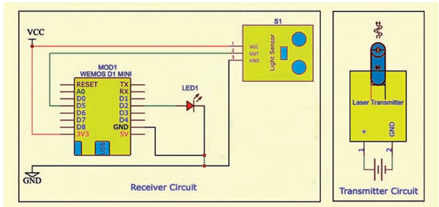
Fig. 3: Circuit diagram
