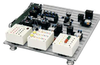
PLC Controlled Electro Pneumatic Training System -
