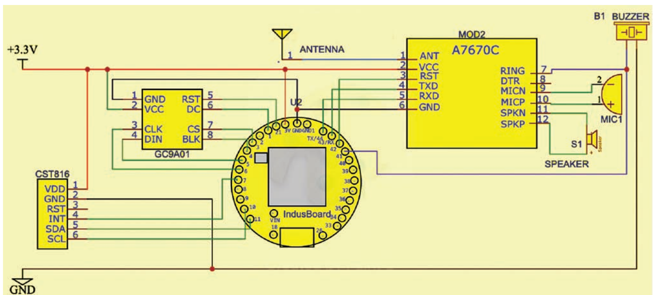
Fig. 3: Circuit diagram
