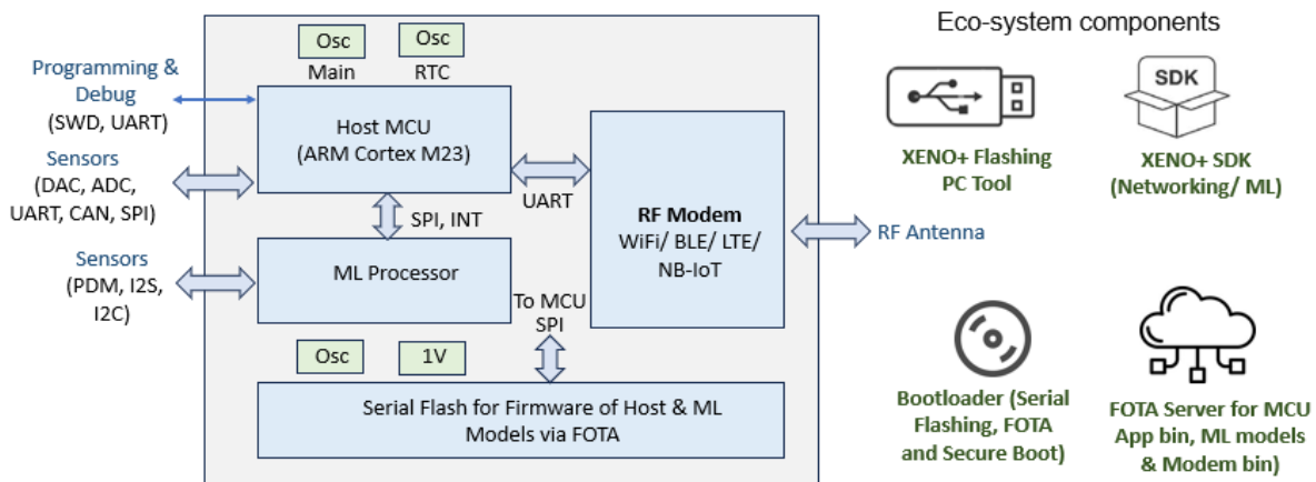
Block diagram of XENO+ ML SOM module and associated eco-system components
