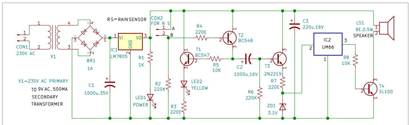
Fig. 2: Circuit diagram
