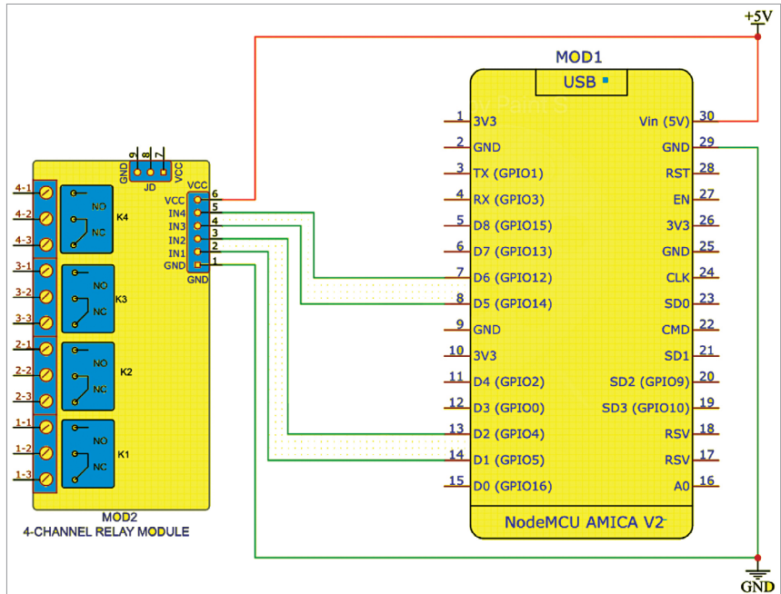
Fig. 2: Circuit diagram
