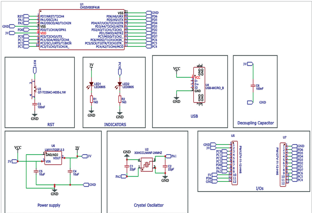
Fig. 5: CH32V00 reference design
