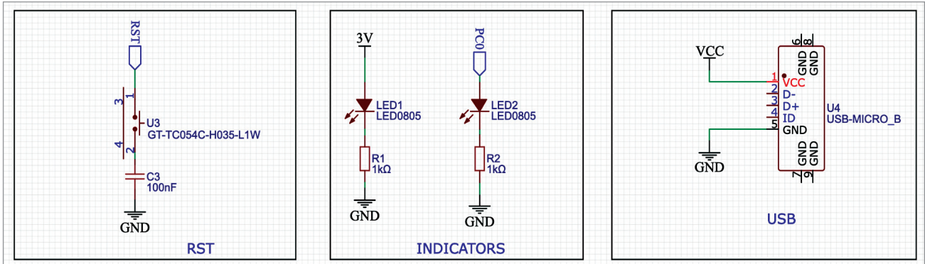
Fig. 3: RISC-V chip circuit configuration
