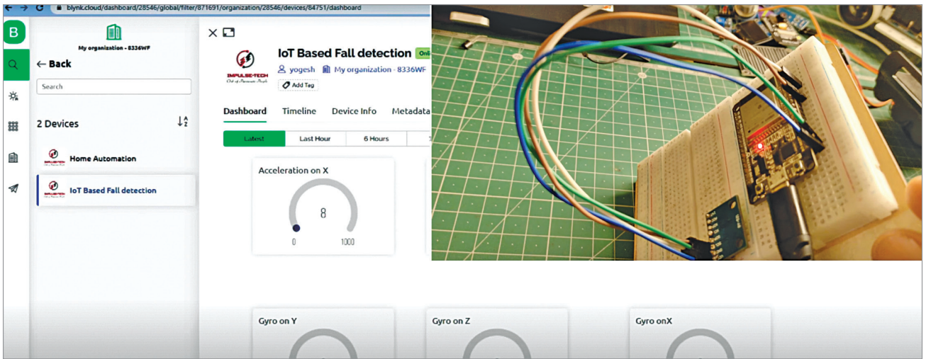
Fig. 3: Blynk dashboard
