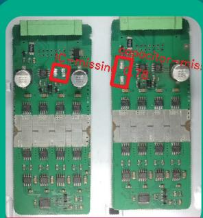
Missing IC/Capacitor
