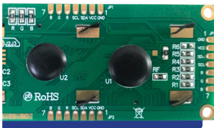
16x2 Display (In-built I2C)
