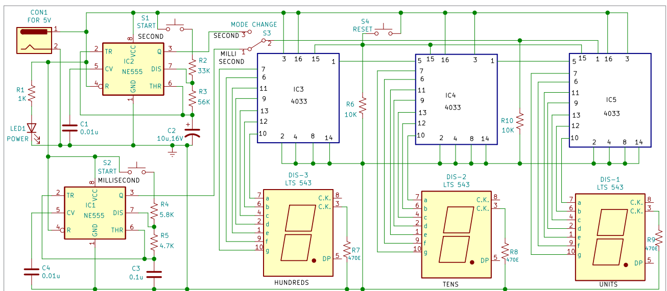
Fig. 2: Circuit diagram
