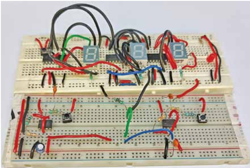
Fig. 1: Author's prototype
