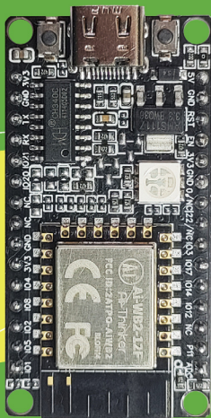
CH340C Board
