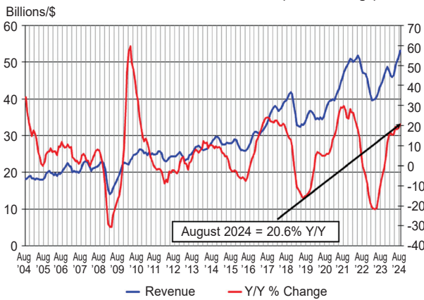
Worldwide Semiconductor Revenues (YoY % Change)
