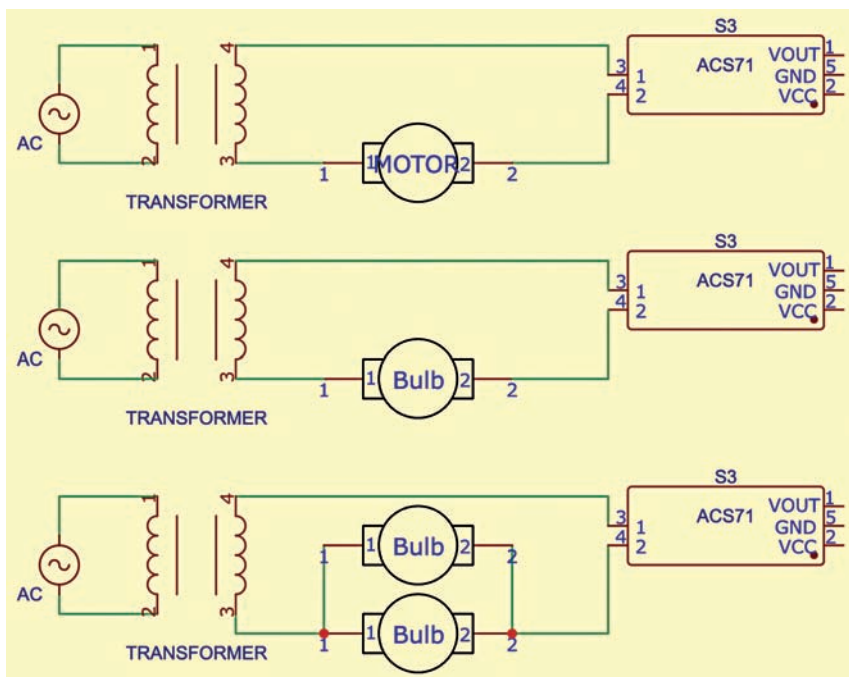
Fig. 7: Various load connection diagrams
