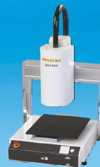
Desktop AOI
