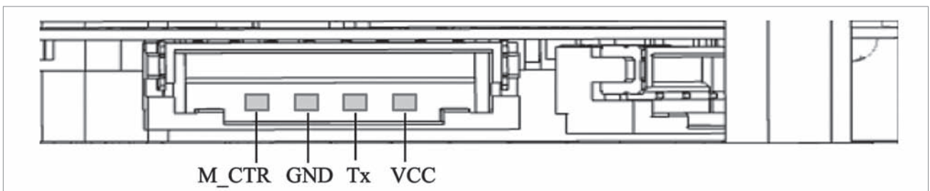
Fig. 3: Lidar connector pins (Source: YD X2 lidar datasheet)
