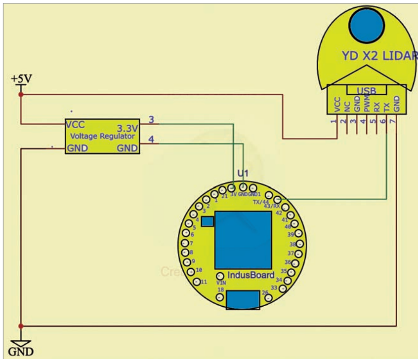
Fig. 4: Circuit diagram
