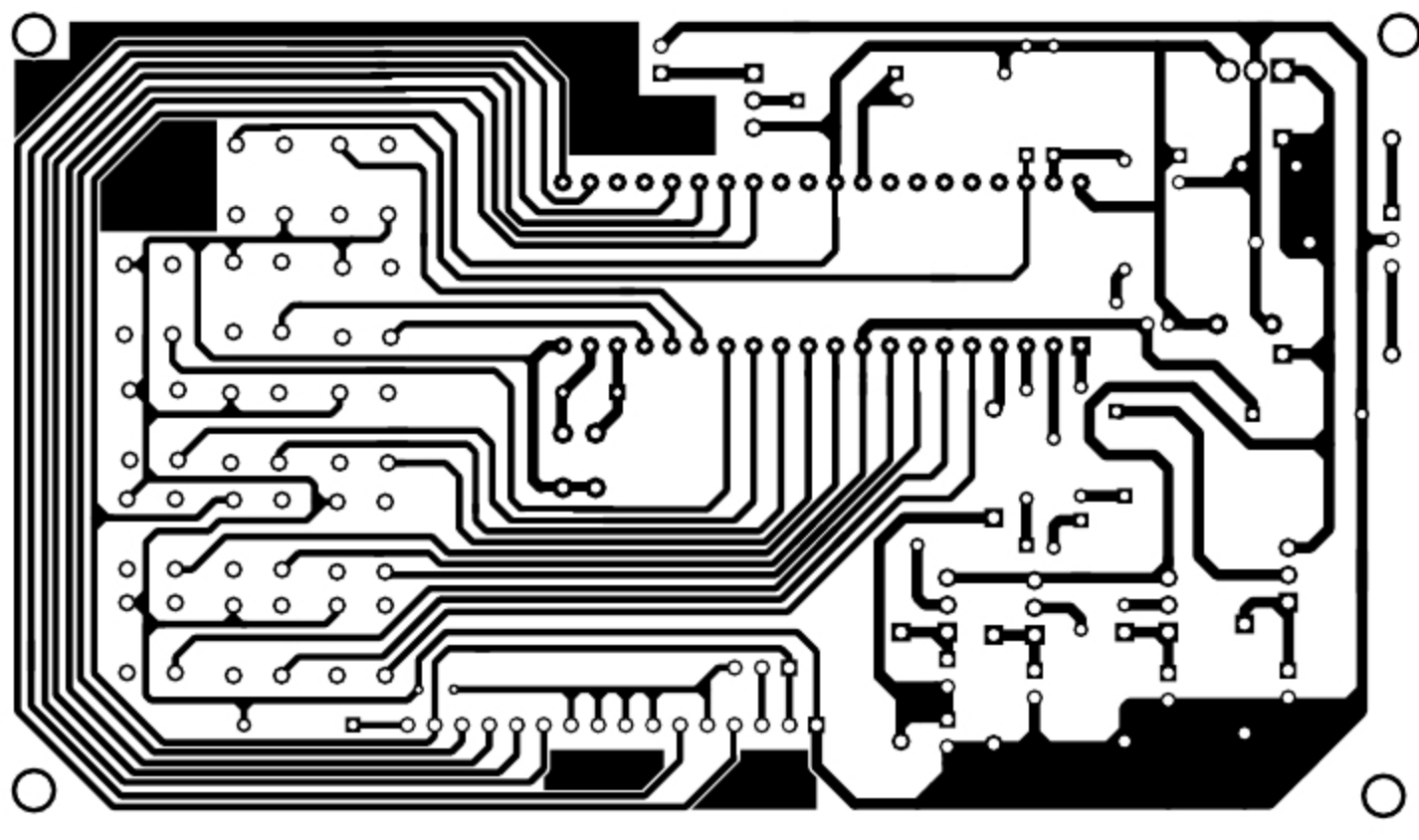
Fig. 3: Actual size PCB layout of microwave oven
