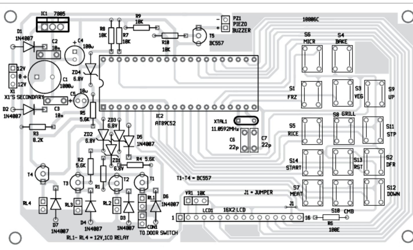
Fig. 4: Components layout for the PCB
