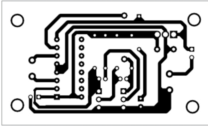
Fig. 4: Actual-size PCB layout of low-cost and versatile hand mixer
