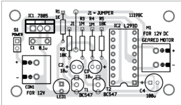
Fig. 5: Components layout for the PCB
