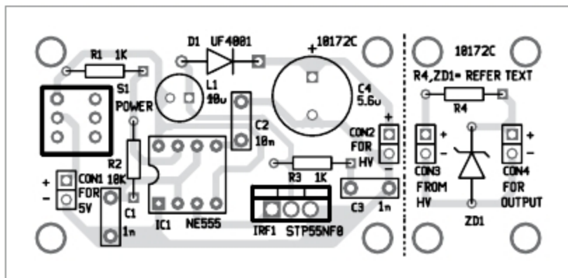
Fig. 4: Components layout for the PCB
