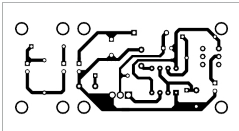
Fig. 3: Actual-size PCB layout of high-voltage generator
