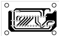
Fig. 3: Actual-size PCB layout of GPS- and GSM-based vehicle tracking system
