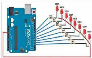
Fig. 3: Circuit diagram of the project
