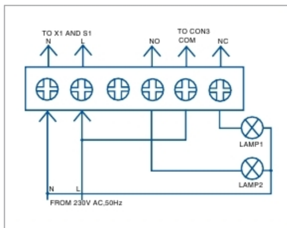
Fig. 6: Lamps connections
