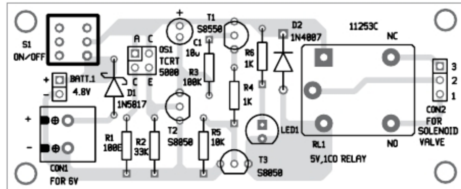
Fig. 4: Components layout for the PCB
