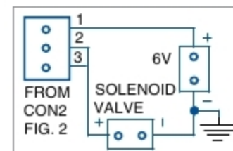
Fig. 6: Wiring diagram of solenoid valve
