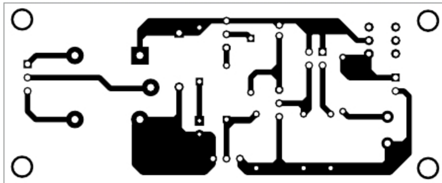
Fig. 3: Actual-size PCB layout of automatic IR faucet controller
