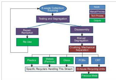
Fig. 1: An overview of e-waste recycling operation (Source: IndigoEdge)
