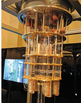
IBM model for universal quantum computer
