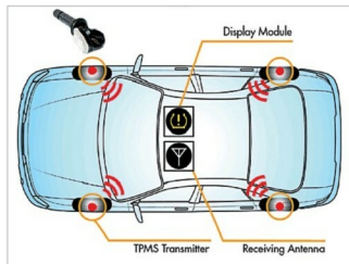
Fig. 7: Overview of TPMS (Courtesy: www.mwrf.com)
