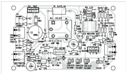
Fig. 9: Components layout for the PCB in Fig. 8
