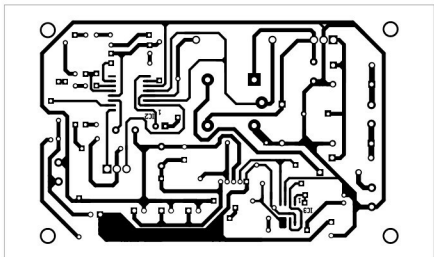
Fig. 8: Actual-size PCB layout of power unit
