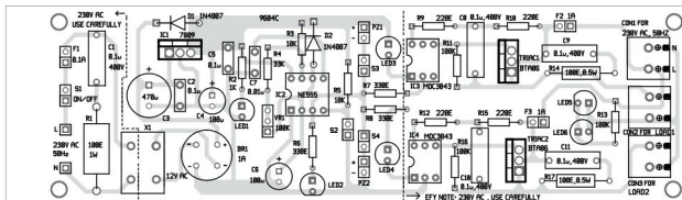
Fig. 3: Components layout for the PCB
