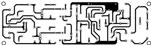
Fig. 2: Actual-size PCB layout of AC lamp blinker
