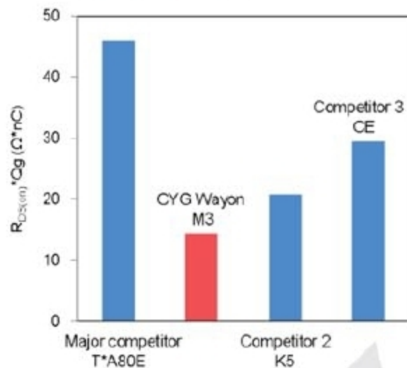
Figure 1. 800V Power MOS FOM comparison
