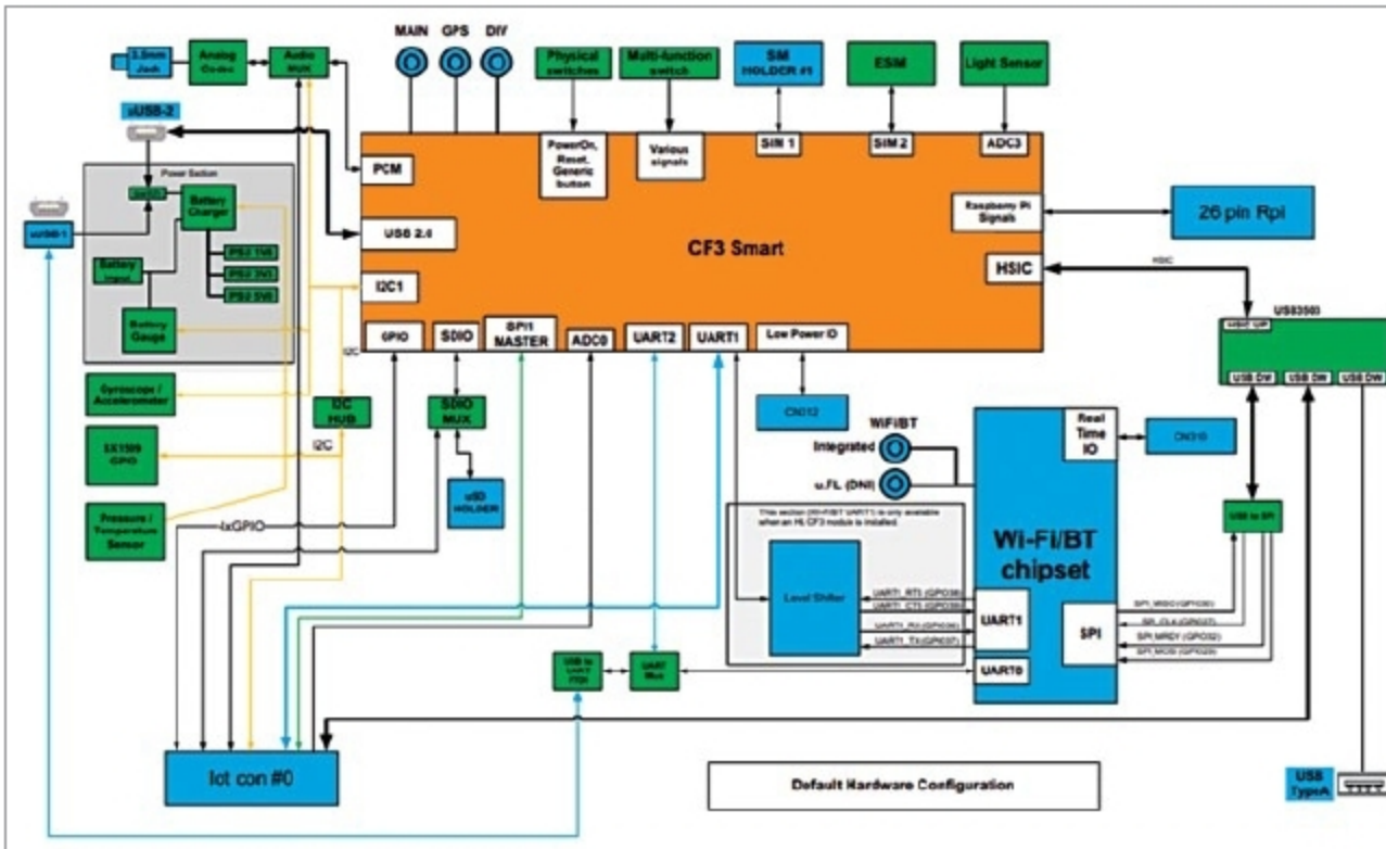
mangOH Red schematic (Credit: https://mangoh.io )
