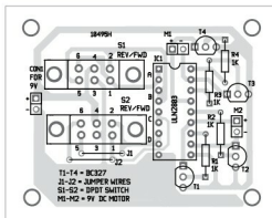
Fig. 3: Components layout for the PCB
