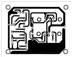
Fig. 2: Actual-size PCB layout of bi-directional DC motor control
