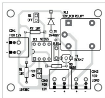
Fig. 4: Components layout for the PCB
