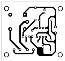
Fig. 3: Actual-size PCB layout of water refiller for air-coolers
