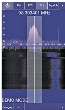
Fig. 6: Spectrum in SDRTouch app
