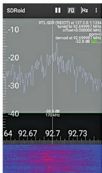
Fig. 11: Spectrum in SDRoid
