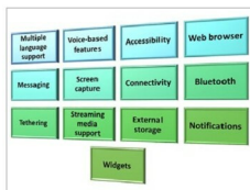
Fig. 2: Android features
