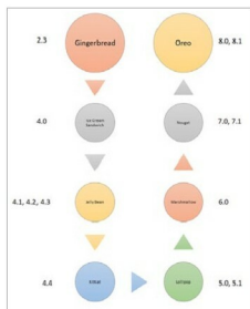
Fig. 1: Android versions
