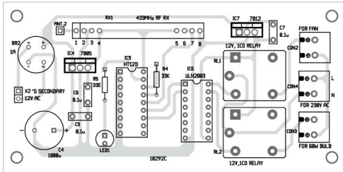
Fig. 8: Components layout for the PCB (receiver section)
