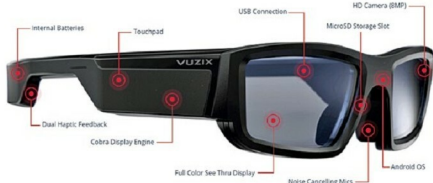
Various features of Vuzix Blade (Credit: www.vuzix.com)
