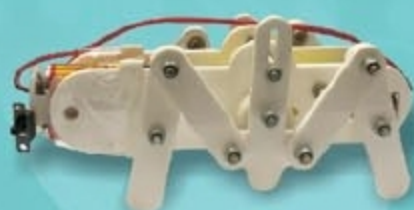
HEXAPOD
