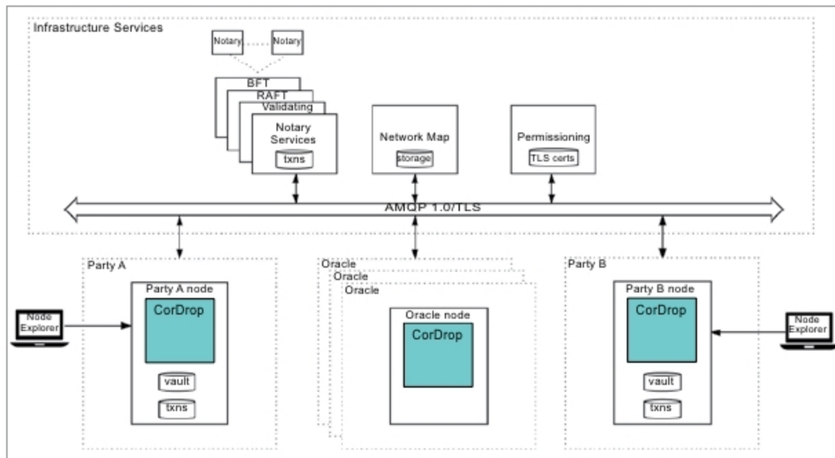
Fig. 3: Components of Corda
