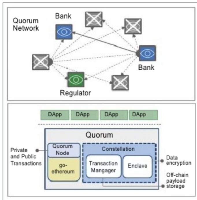
Fig. 4: Quorum network architecture
