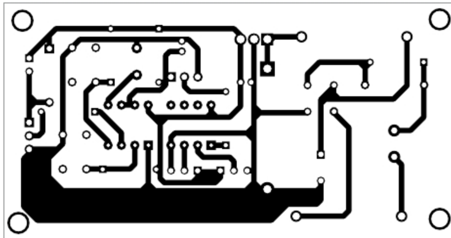
Fig. 2: Actual-size PCB layout of washbasin mirror light controller
