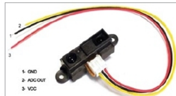
Fig. 4: Sharp 2Y0A21 sensor
