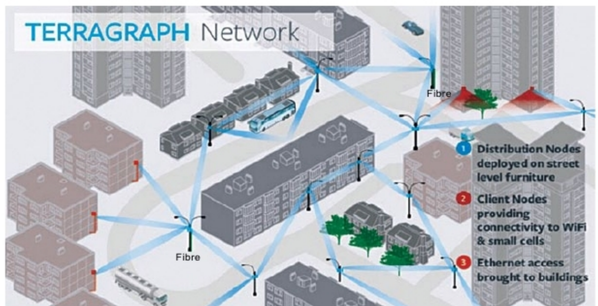
Terragraph network by Facebook
