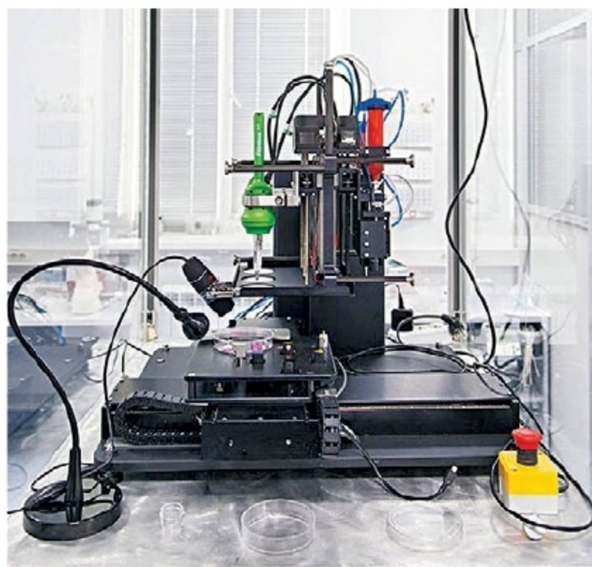
Fig. 2: Printer from Russia-based 3D Bioprinting Solutions (Credit: Wikipedia)
