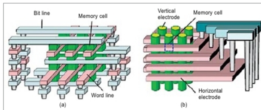
Fig. 3: A non-linear ReRAM cell with sub-1 \mu A ultra-low operating current for high density vertical resistive memory (Credit: www.semanticscholar.org )
