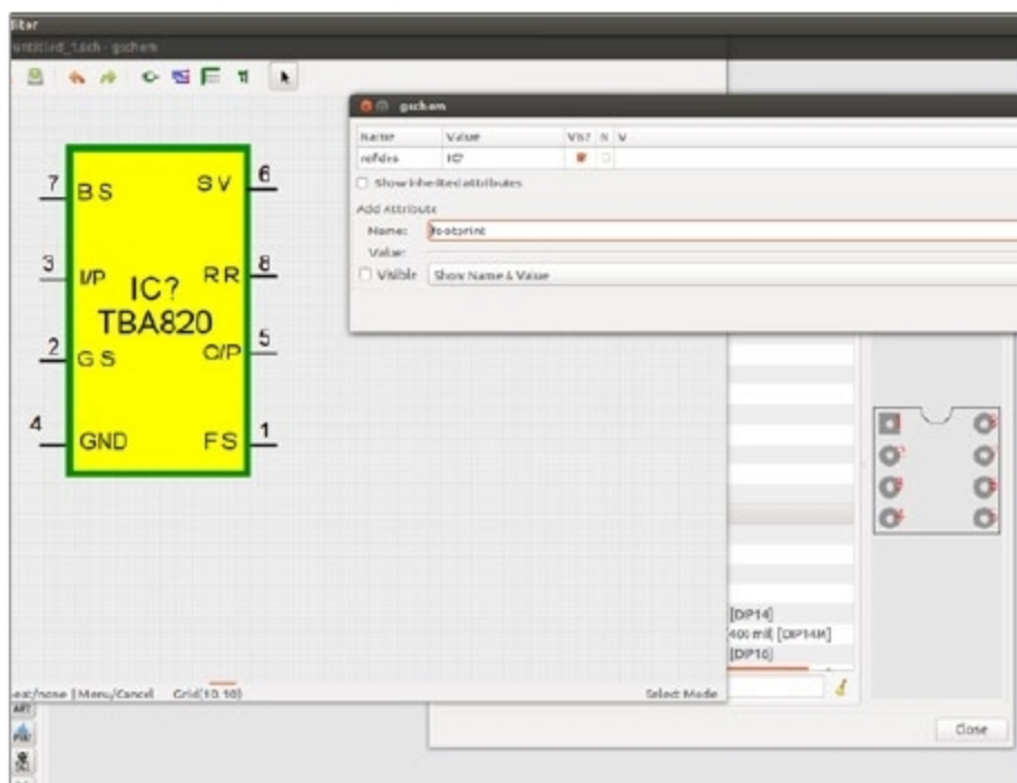
TBA820M footprint in gEDA software
