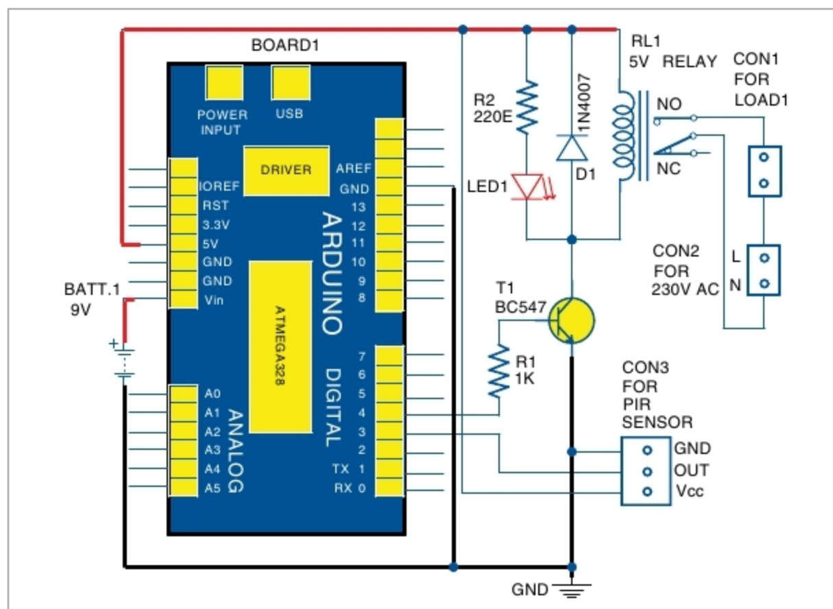
Fig. 1: Circuit diagram of the motion-sensor-based security alert system
